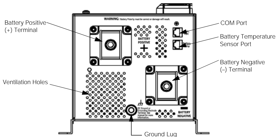
Figure 1-3 DC Side of the Xantrex TR Series
