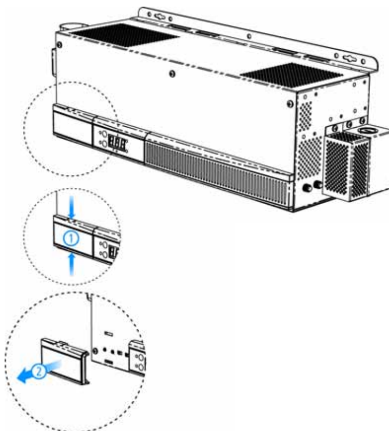
Figure 2-2 Removing the Service Access Cover
